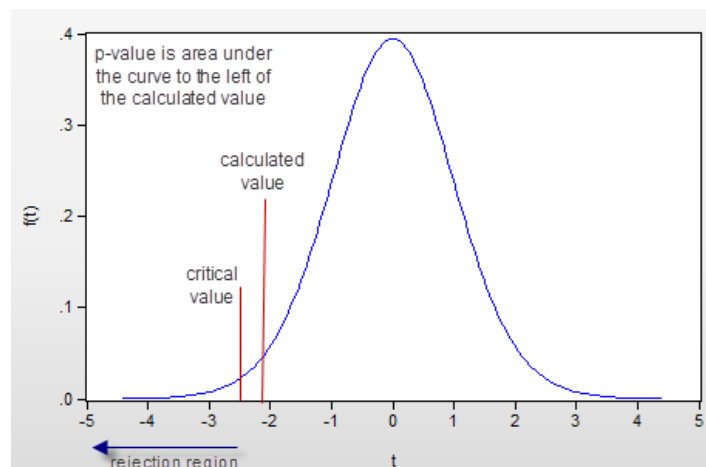
Figure xr3.6(b) Rejection region and p -value
