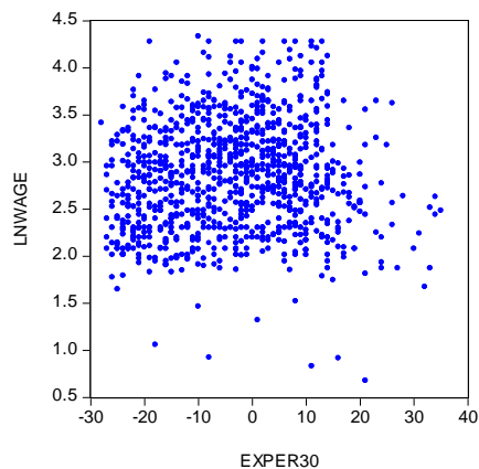
Figure xr3.13(a) Scatter plot of \ln(WAGE) against EXPER30
